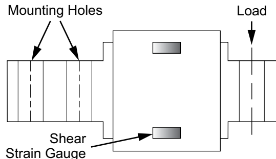
Figure 1-4. Cantilever Beam
