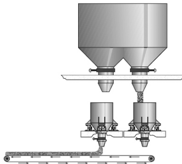
Figure 13-9. Dual Weigh Hopper System
