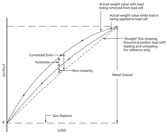
Figure 6-1. Calibration Curve
