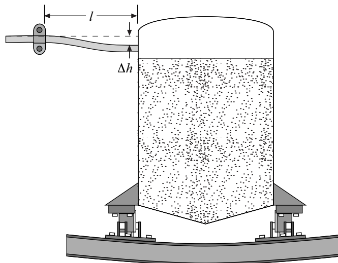
Figure 19-2. Deflection of Vessel Application
