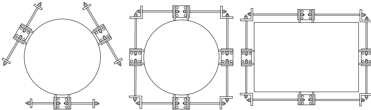
Figure 21-1. Stay Rod Applications
