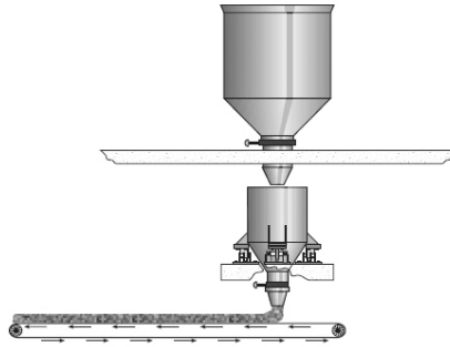
Figure 13-6. Storage Silo Fed Weigh Hopper
