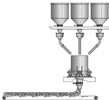
Figure 13-3. Single Weigh Hopper
