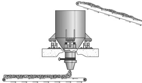
Figure 13-4. Controlled Rate Weigh Hopper
