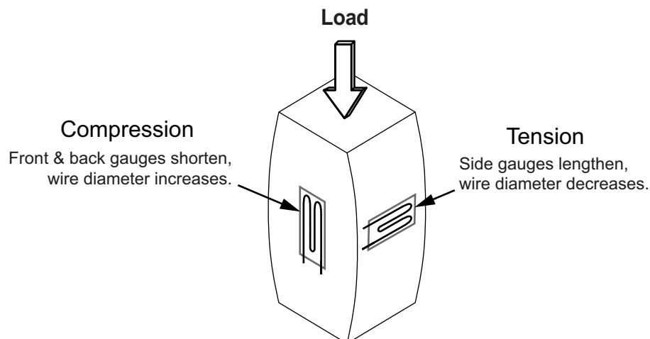
Figure 5-4. Strain Gauge
