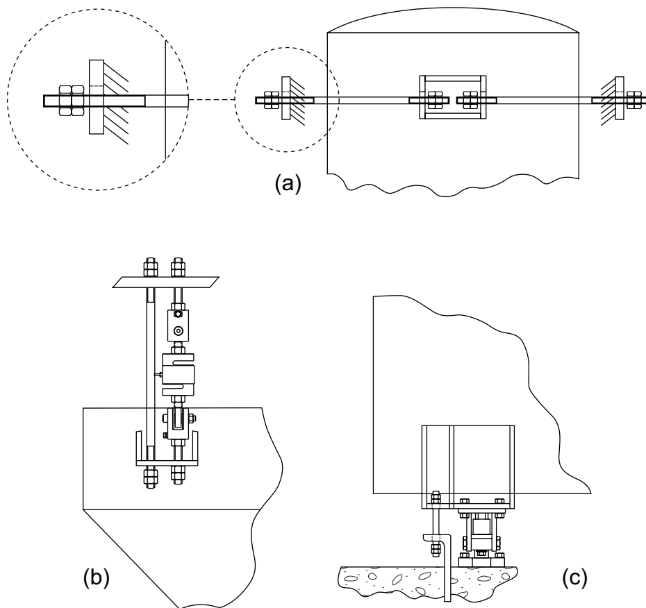
Figure 21-3. Safety Check Rods
