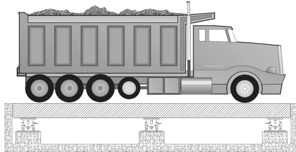
Figure 13-1. Truck Scale Application
