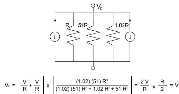
Figure 24-5. Norton Equivalent Circuit with Additional Resistor
