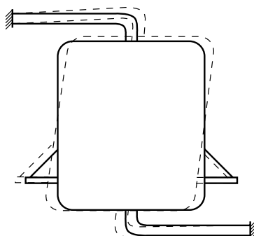
Figure 16-5. Weigh Vessel with Rigidly-Attached Piping
