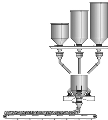
Figure 13-11. Single Weigh Hopper, Multiple-Ingredient Batching System
