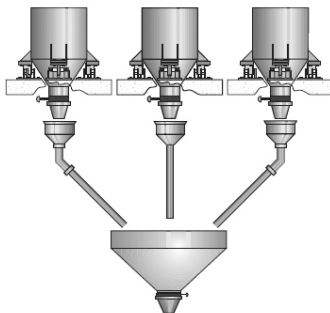
Figure 13-2. Separate Weigh Hoppers
