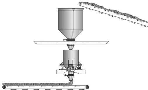
Figure 13-7. Surge Hopper Fed Weigh Hopper
