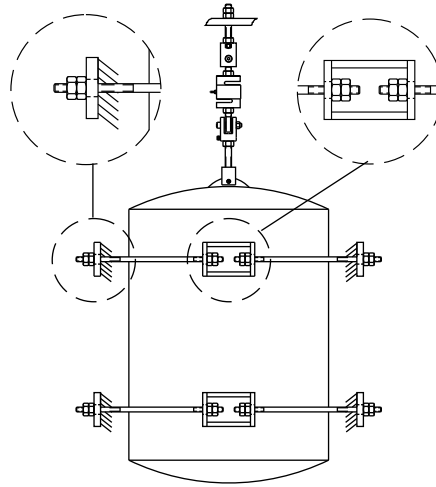
Figure 21-2. Stay Rod Application
