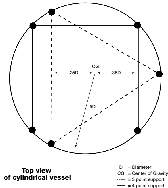
Figure 18-2. Vertical Cylindrical Vessel Top View
