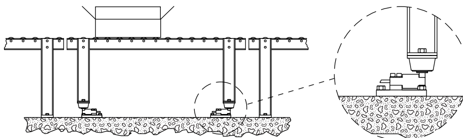
Figure 8-6. RL50225TA on Conveyor
