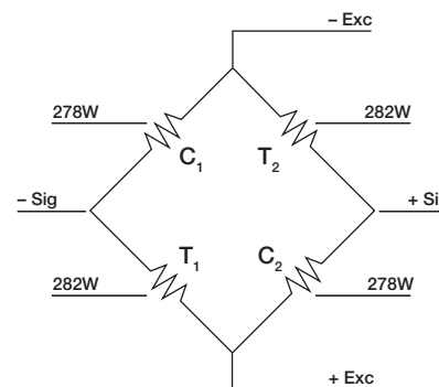
Figure 25-2. Wheatstone Bridge
