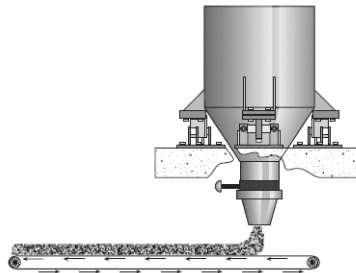
Figure 13-10. Loss-in-Weight System
