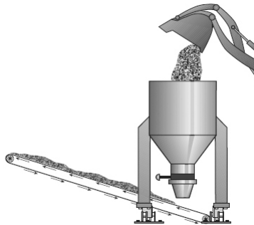
Figure 13-5. Loader Fed Weigh Hopper
