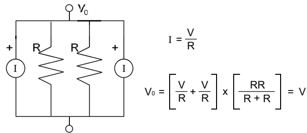
Figure 24-4. Norton Equivalent Circuit
