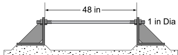
Figure 16-2. Stay Rod
