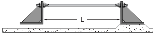
Figure 16-1. Stay Rod
