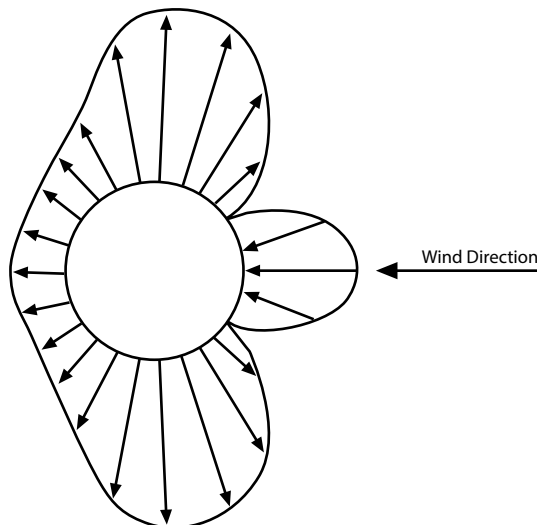
Figure 18-3. Wind Forces on a Vertical Cylindrical Vessel
