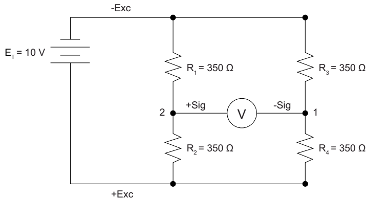
Figure 6-3. Wheatstone Bridge
