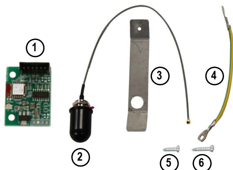
Figure 1. Retrofit Kit (212110)
