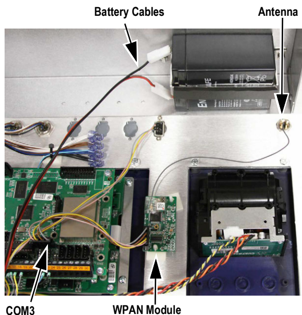
Figure 8. Removing WPAN Module
