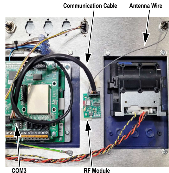
Figure 10. Install RF Module
