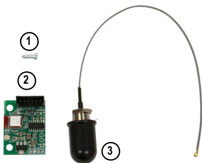
Figure 6. Ai-1 Indicator RF Retrofit Kit Parts (212111)
