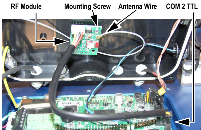
Figure 5. RF Module Installation
