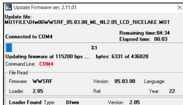
Figure 2. Firmware Update Status Window
