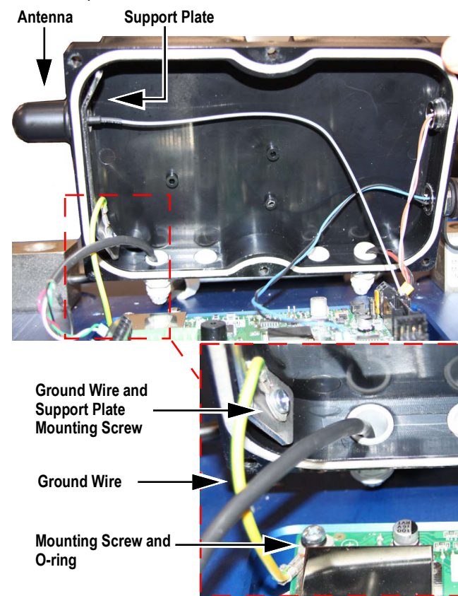
Figure 4. Antenna and Ground Wire Installation
