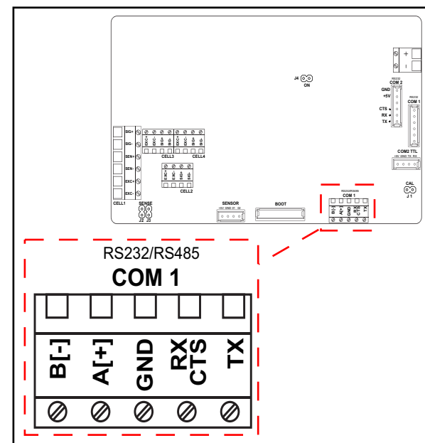
Figure 4. Wheel Weigh Pad Serial Port
