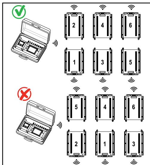
Figure 6. Wheel Weigh Pad Positioning
