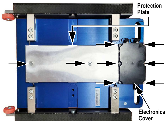
Figure 2. Protection Plate and Cover Mounting Bolts
