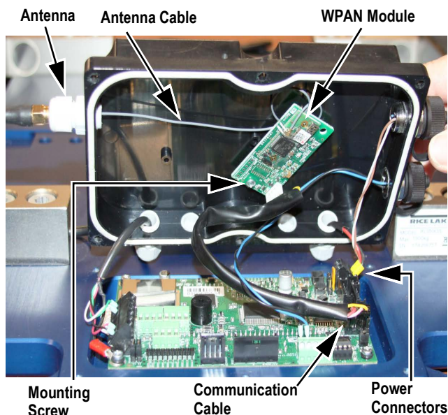
Figure 3. Existing Hardware Removal
